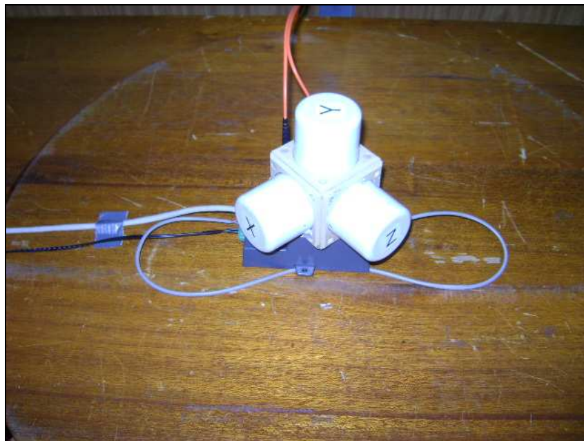
SANS / IEC 61000-4-3: Radiated immunity test set-up
