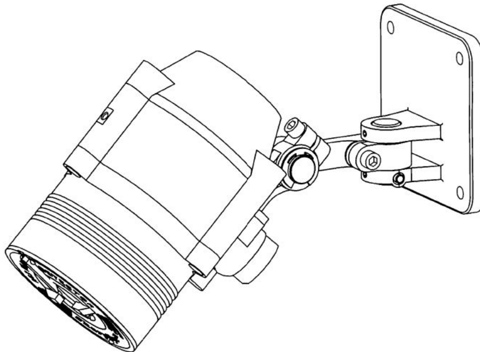
Figure 17: Tilt Mount
