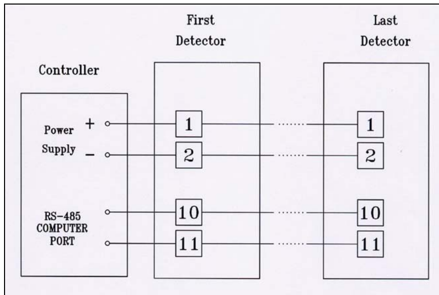
Figure 14: RS-485 Networking
