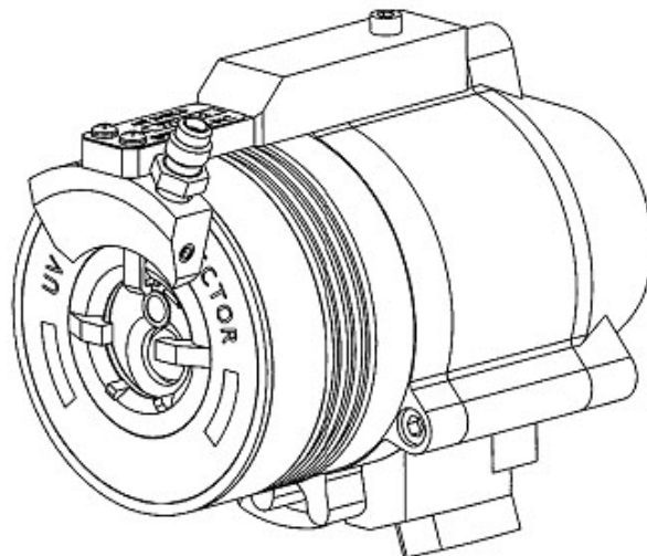
Figure 20: Air Shield
