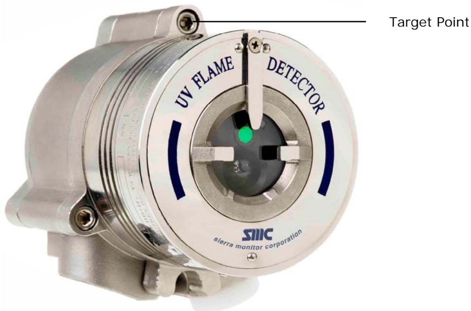
Figure 16: 3600U and UB Detector Target Point
