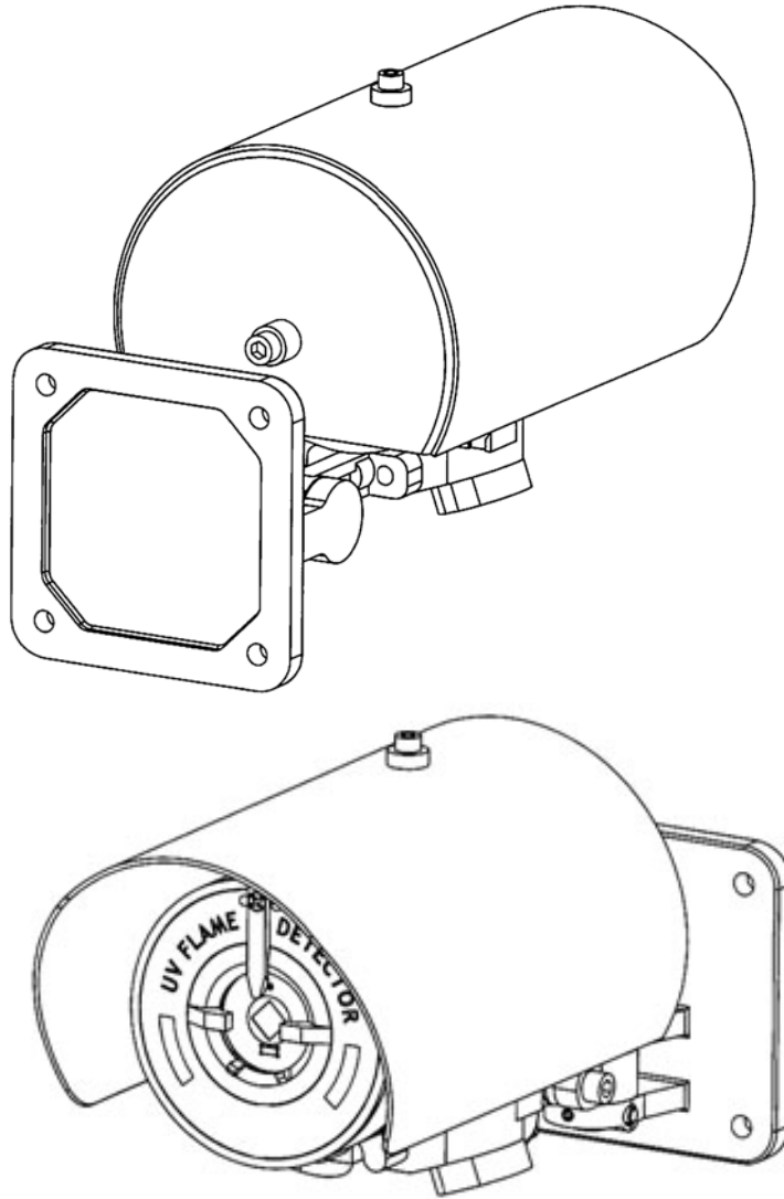
Figure 18: Weather Protection
